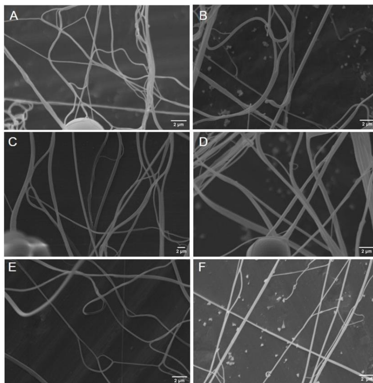
Figure 1. Scanning electron microscopy of nanofibers containing: (a) CO: LO – 100:0, (b) CO: LO – 75:25, (c) CO: LO – 50:50, (d) CO: LO – 25:75, (e) CO: LO – 0:100, (f) PLA nanofibers.
