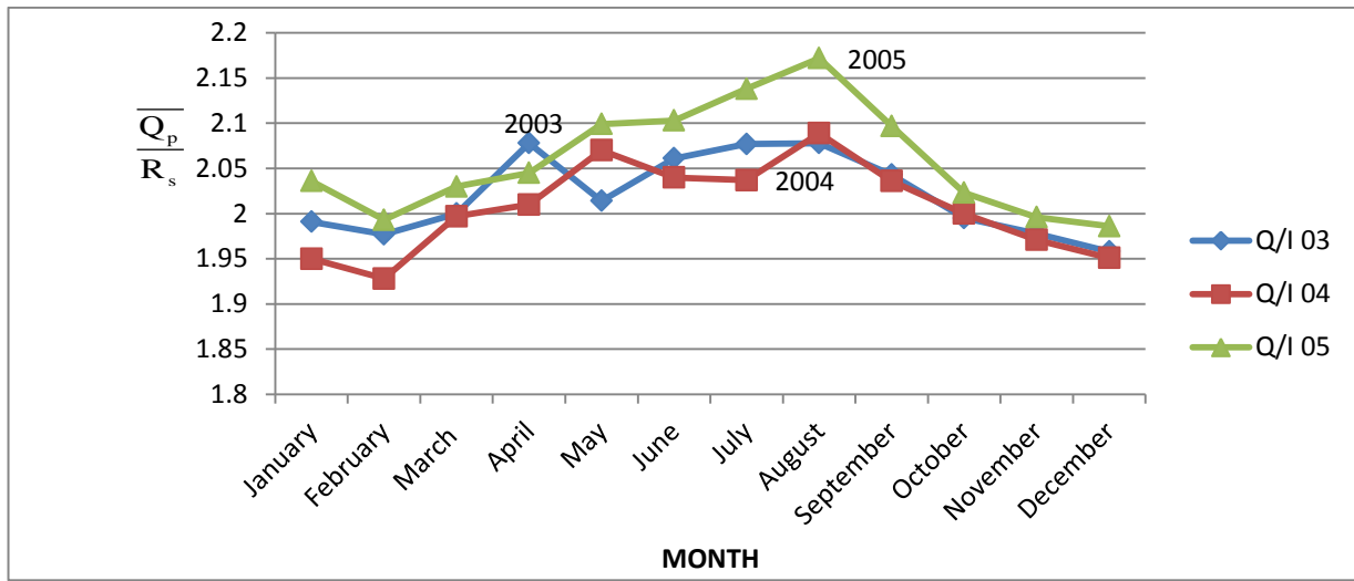
Fig-6. Variation of Mean Monthly Ratio of Hourly Par, Q_p to Hourly Global Solar Radiation, R_s .
