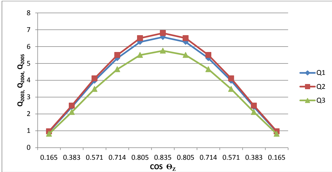
Figure-5. Variation of Estimated Par, Q_p for December 2003, 2004 and 2005 with cosine of Zenith Angle, \text{Cos } \Theta_z
